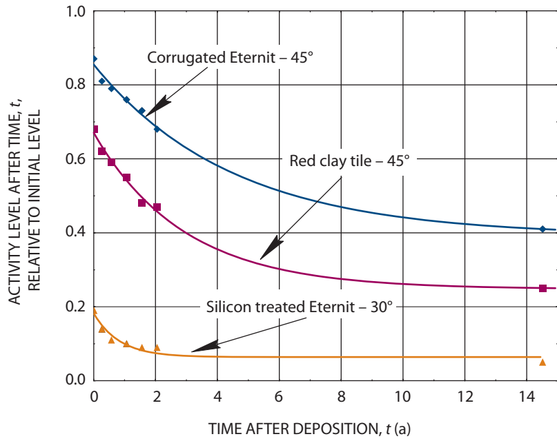
Figure A-VI. Measured ^{137}\text{Cs} activity levels (relative to the initial deposition on soil) on three types of roof at Risø, Denmark [A6]
