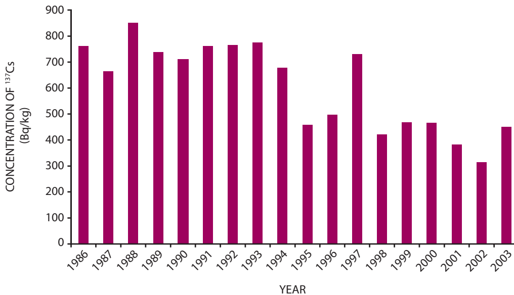
Figure A-XVIII. The average concentration of 137 Cs in moose in one hunting area in Sweden
