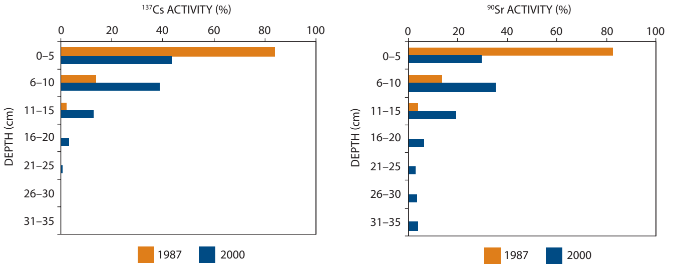
Figure A-X. Depth profiles for 137 Cs and 90 Sr measured in 1987 and 2000 in a soddy-gley-sandy soil (in % of total activity) [S14]
